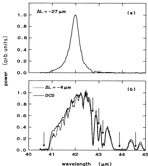
FIG. 2. Power spectrum corresponding to the three cases shown in Fig. 1(a). The arrows indicate absorption lines in ambient water vapor in the spectrometer setup. The spectra are integrated over the macropulse. Each spectrum is measured by scanning the spectrometer during 200 successive macropulses. The power scale is different in (a) and (b).
