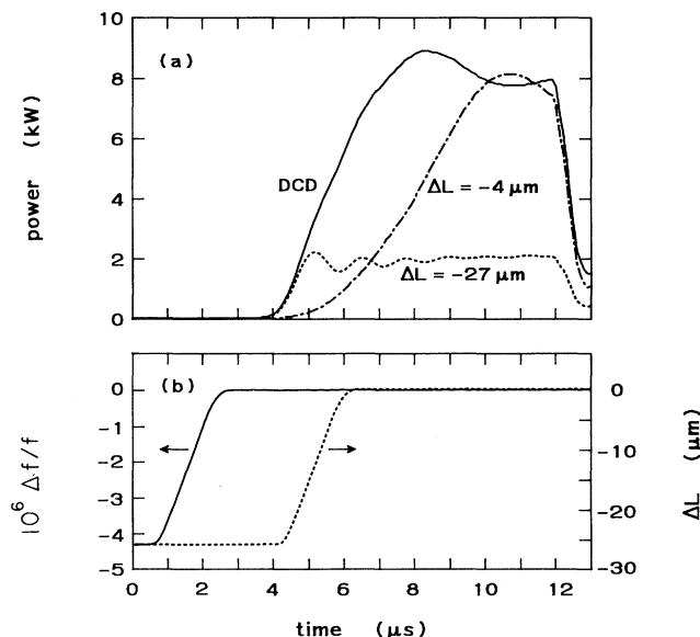
FIG. 1. Optical macropulses measured at a wavelength of 42 \mu\text{m} (a), as obtained at a fixed cavity desynchronism giving a large single-pass gain ( \Delta L = -27 \mu\text{m} ), at a desynchronism giving a large saturated power ( \Delta L = -4 \mu\text{m} ), and with the dynamic cavity desynchronization (DCD) shown in (b). The electron beam macropulse starts at t=0 , the beaming-loading transient in the accelerator has died out at t=1.5 \mu\text{s} , and the macropulse ends at t=12 \mu\text{s} . The full line in (b) gives the applied ramp signal to the FM input of the maser oscillator. The dotted line gives the equivalent cavity length detuning, when the observed 3.5\text{-}\mu\text{s} delay in response of the rf system is taken into account.
